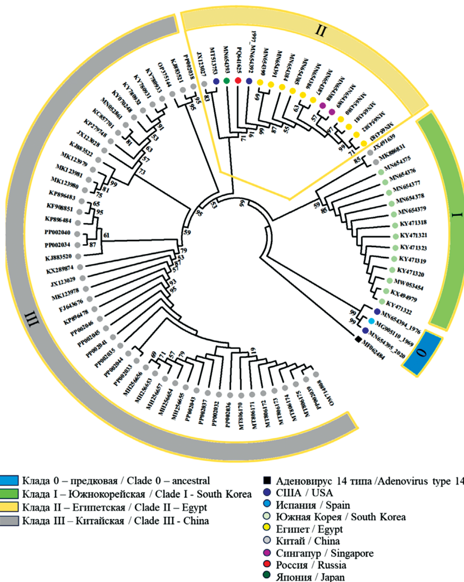
Fig. 2. Neighbor-joining phylogenetic tree constructed based on the complete genomes of 83 HAd-55 isolates presented in Table 1, and the genome of the SCV3008:Ad55 isolate (PQ641625).
